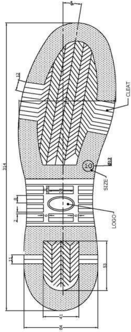
BOTTOM VIEW
